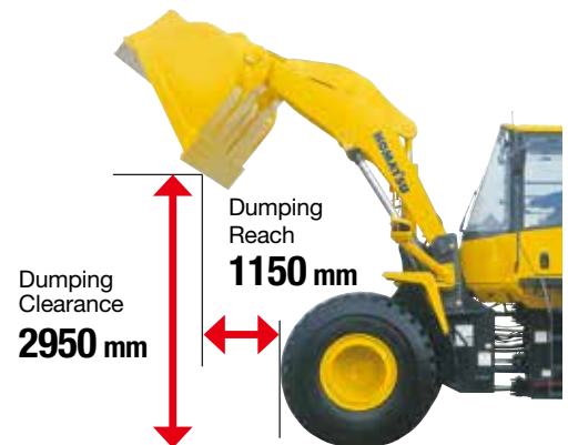
(3.3m 3 bucket with Bolt on cutting edge (B.O.C.))
